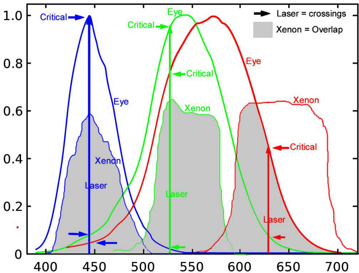
Figure 3. Overlap between spectral sensitivity and Xenon, and crossings with laser. Source: http://www.kommer.com/20230616_Kommer_Kleijn_Laser_def.pdf
